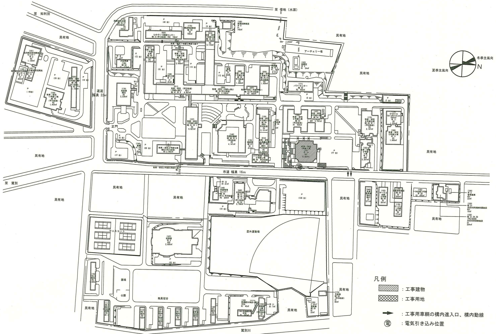
縮尺 S=1/3,000
